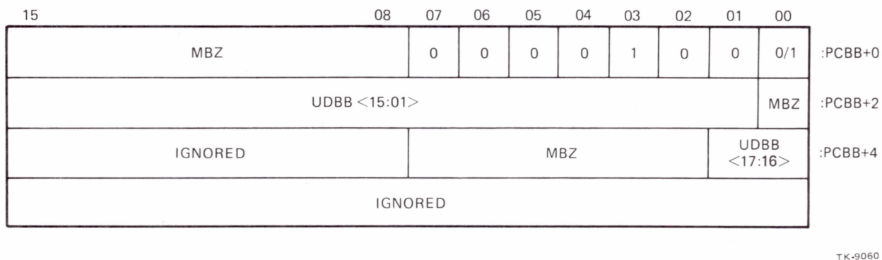
Figure 4-12 Read/Write Descriptor Ring Format, Ancillary Function Codes 10/11 Bit Format
