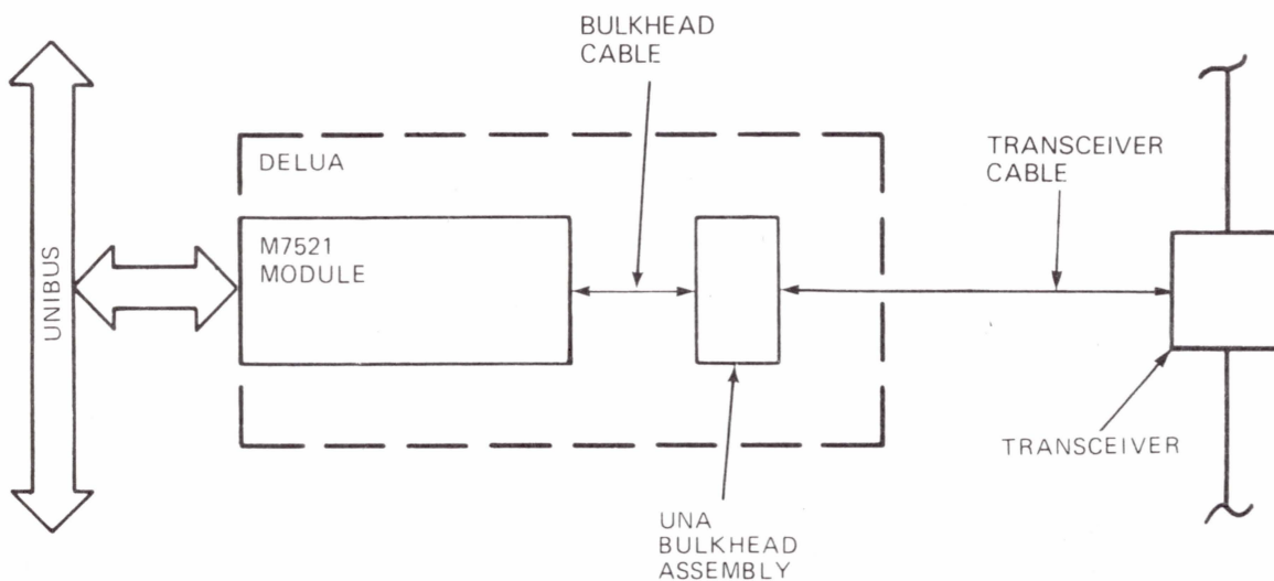
Figure 1-3 DELUA-to-LAN Block Diagram
