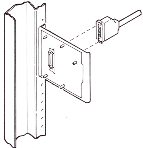
Figure 2-8 DELUA Installation Procedure (Sheet 2 of 2)
