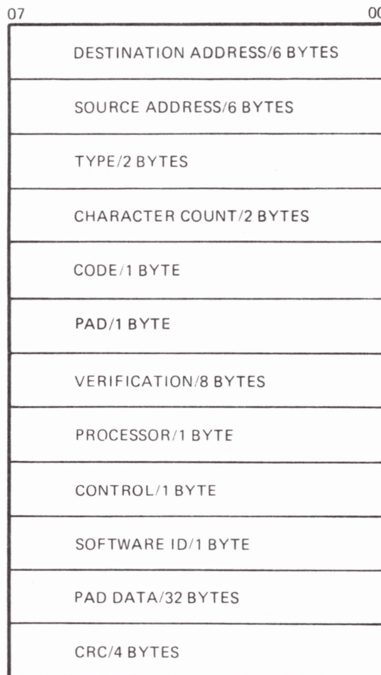
Figure 5-1 Boot Frame Format
