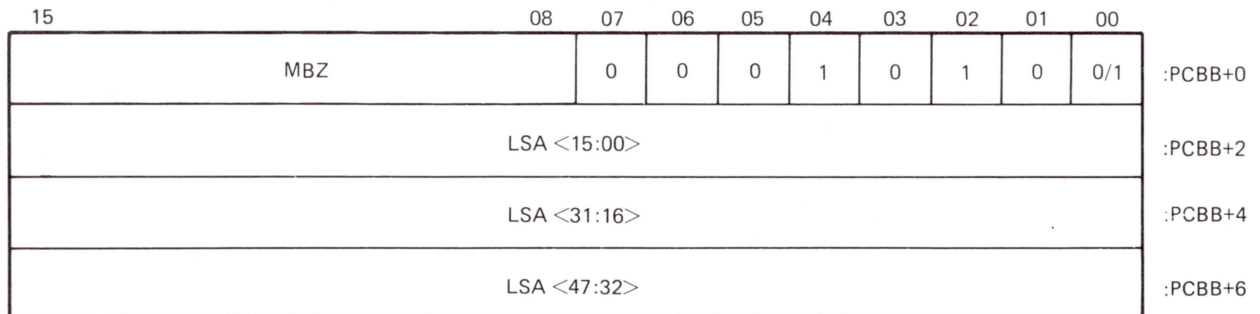
Figure 4-22 Read/Write Load Server Address, Ancillary Function Codes 24/25 Bit Format
