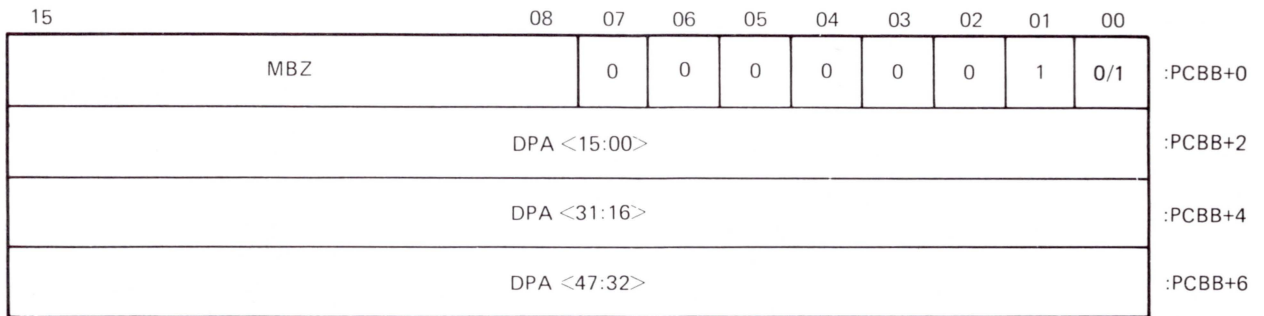
Figure 4-8 Read Default Physical Address, Ancillary Function Code 2 Bit Format
