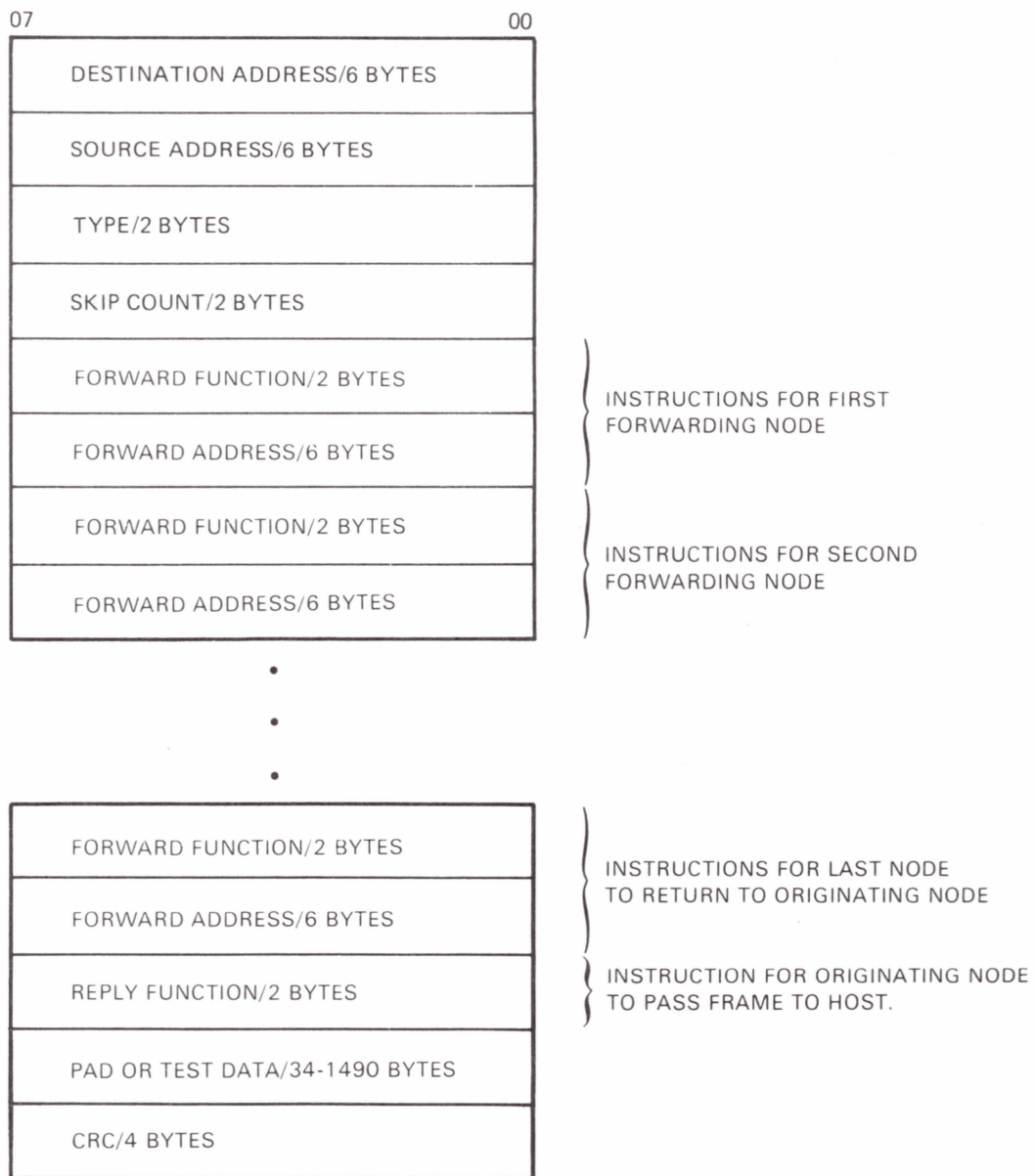
Figure 5-4 Loopback Frame Format
