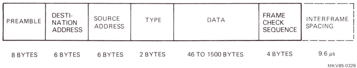
Figure 1-4 Format of a Data Frame
