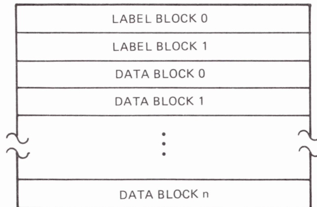
Figure 5-7 Microcode Patch File Format
