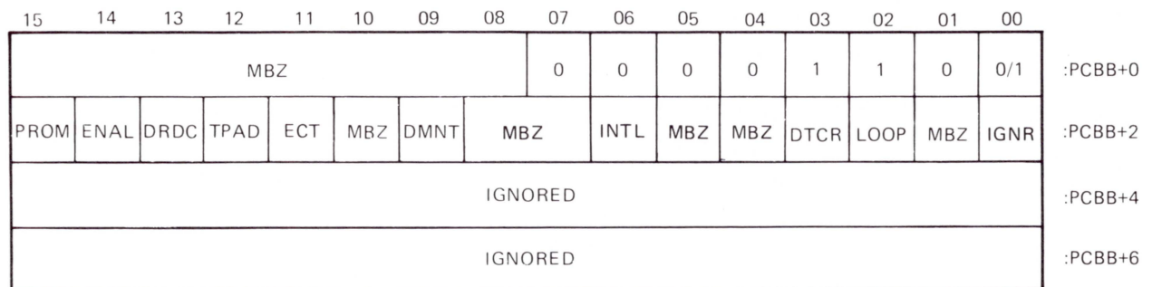
Figure 4-16 Read/Write Mode Register, Ancillary Function Codes 14/15 Bit Format
