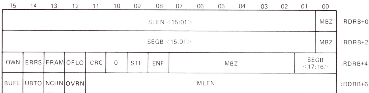
Figure 4-24 Format of an Entry in the Receive Descriptor Ring
