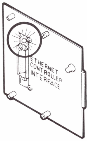
Figure 2-11 Bulkhead LED
