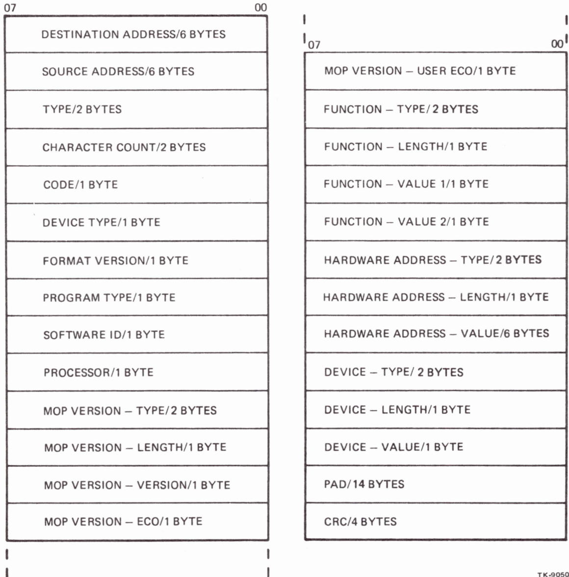
Figure 5-2 Request Program Frame Format
