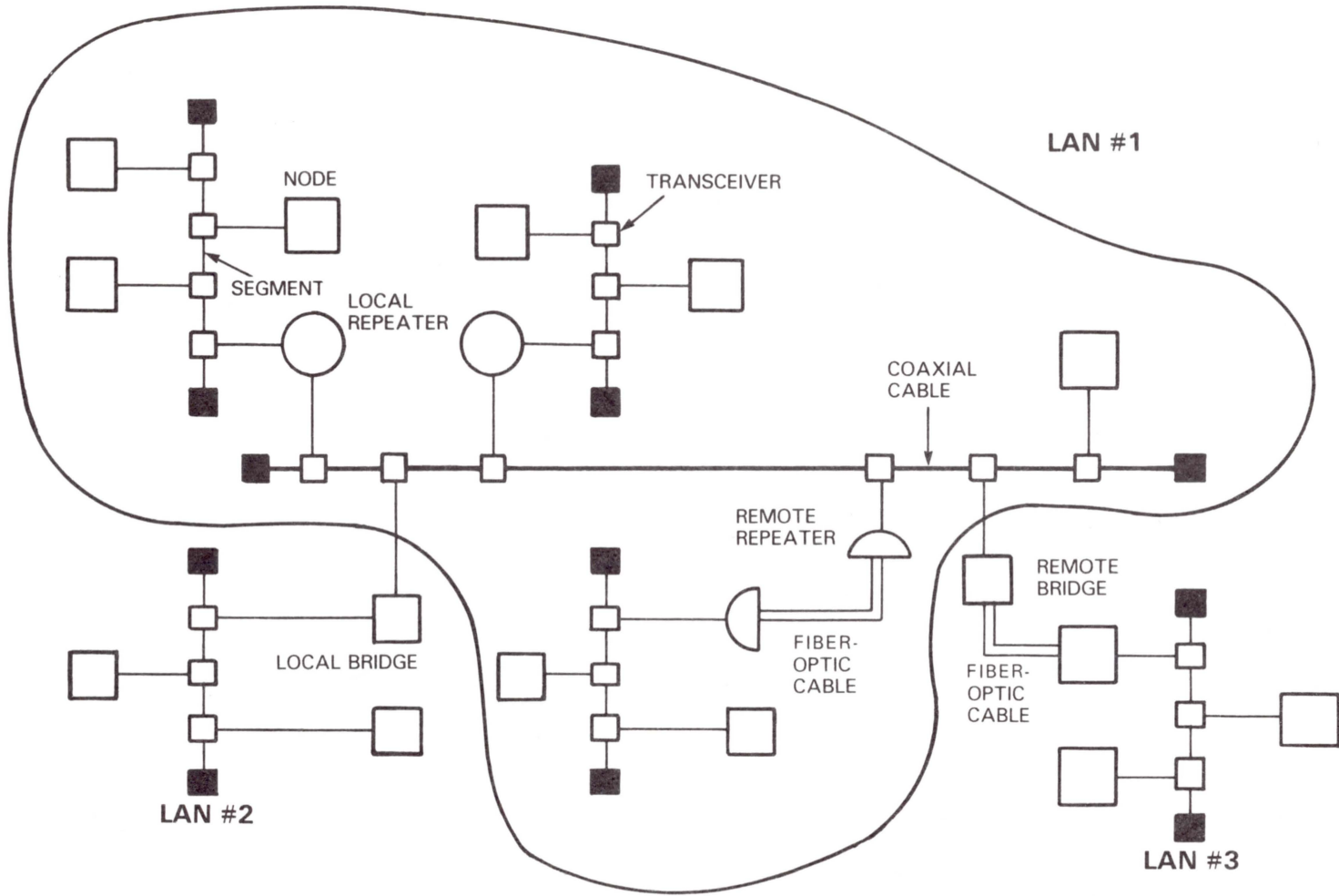
Figure 1-1 Large-Scale Ethernet Configuration
