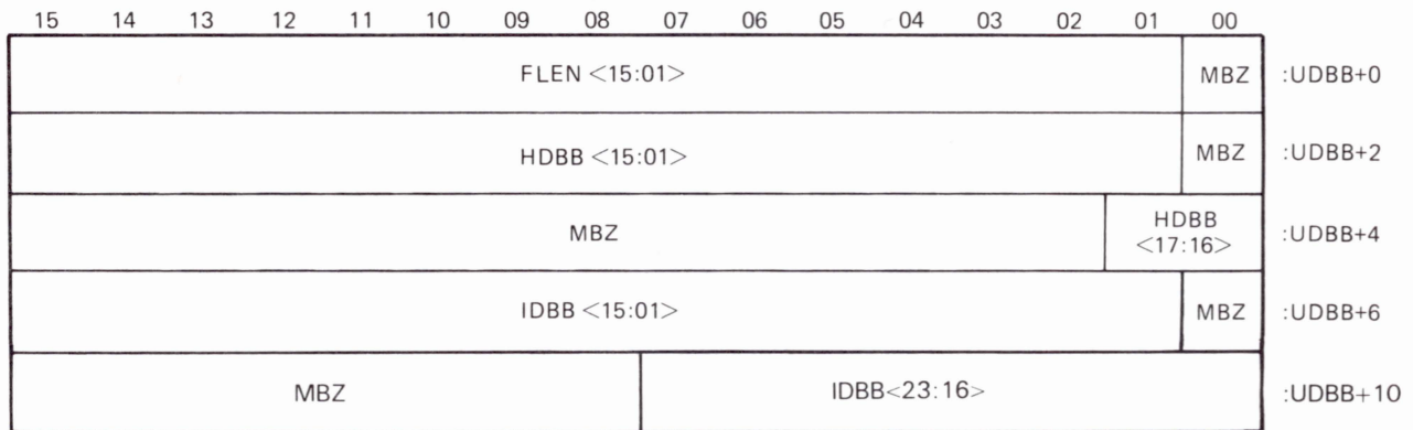
Figure 4-19 Dump/Load Internal Memory UDB Bit Format
