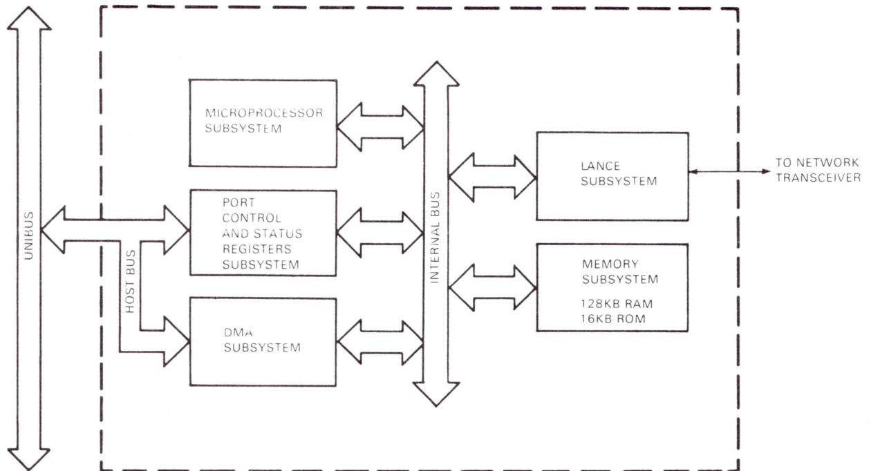
Figure 1-5 DELUA Block Diagram
