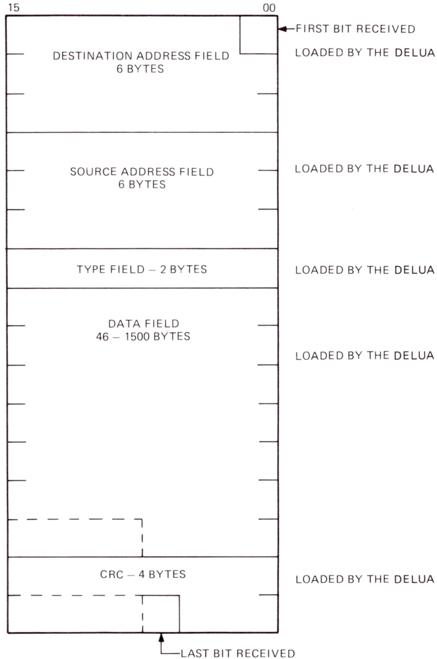
Figure 4-27 Receive Data Buffer Format
