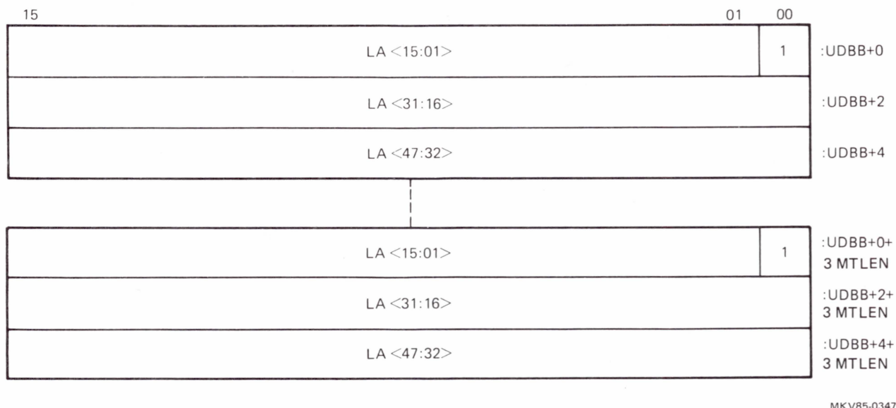
Figure 4-11 Multicast Address List UDB Bit Format
