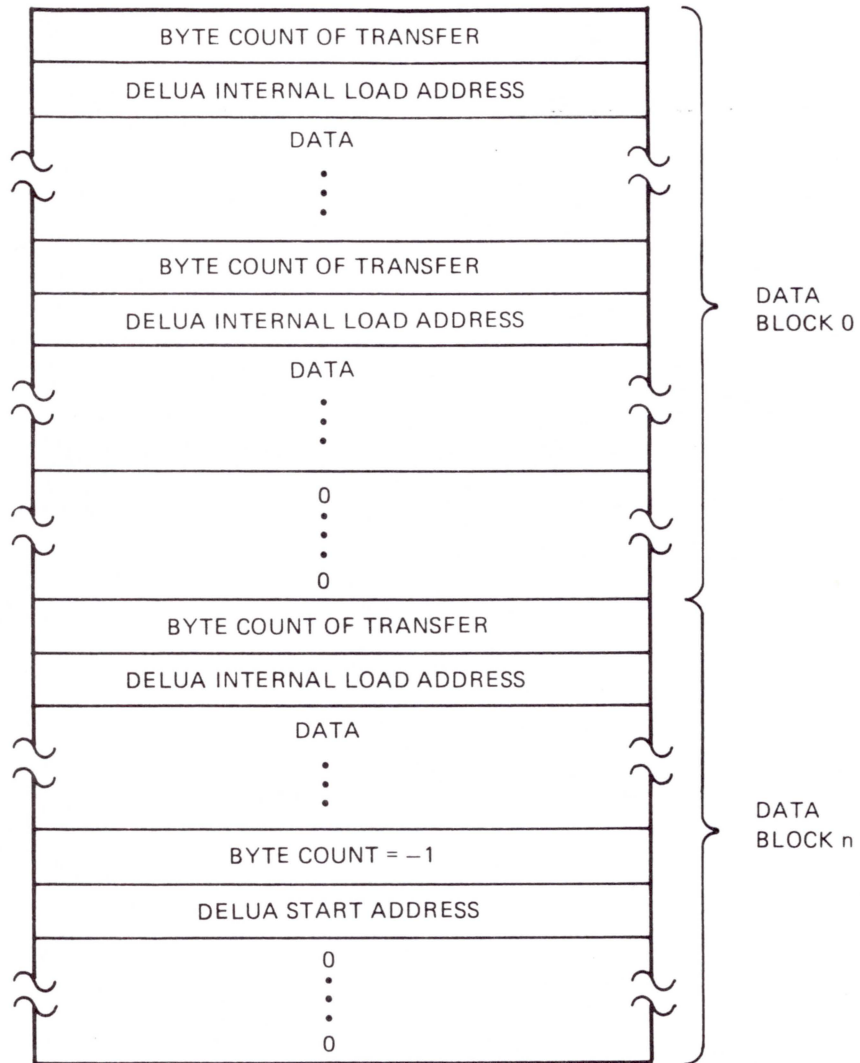
Figure 5-8 Patch File Data Block Format
