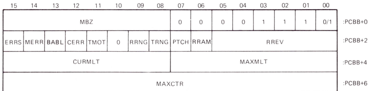
Figure 4-17 Read/Read and Clear Status, Ancillary Function Codes 16/17 Bit Format
