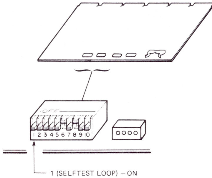
Figure 2-7 Loop Selftest Switch Setting
