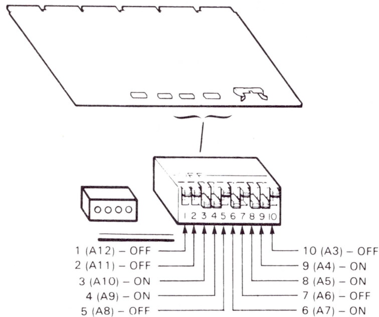
Figure 2-2 Switch Pack at E106, Device Address Assignment
