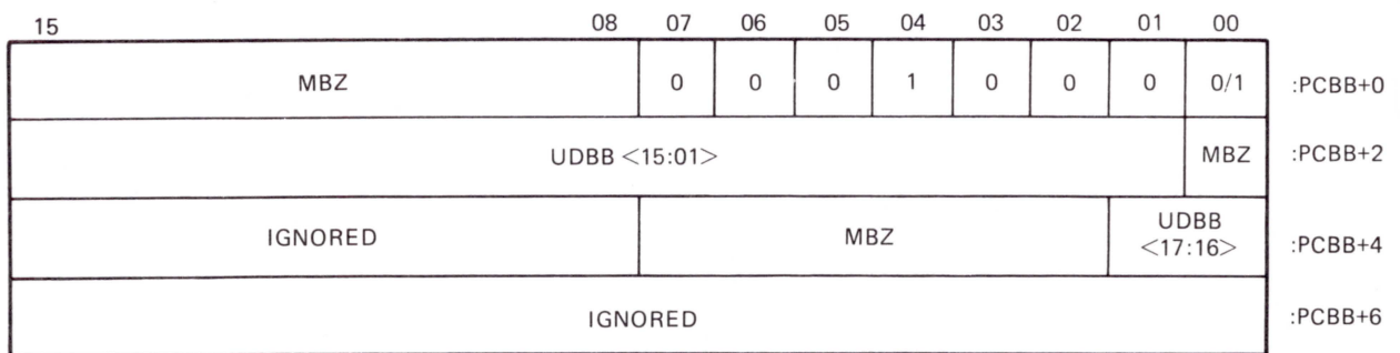
Figure 4-18 Dump/Load Internal Memory, Ancillary Function Codes 20/21 Bit Format
